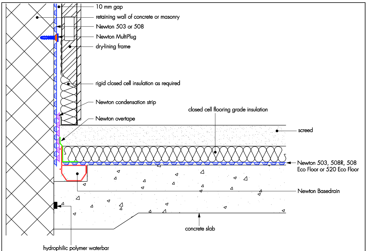
Figure 3 Installation detail
