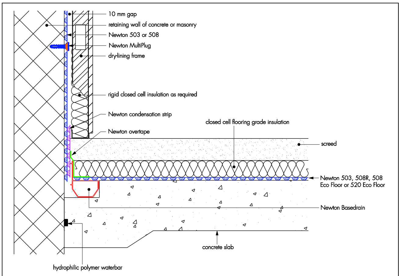
Figure 3 Installation detail
