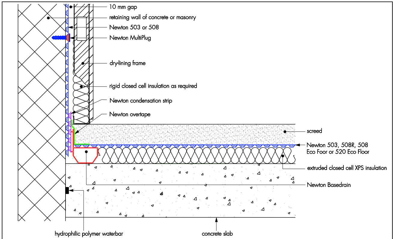
Figure 3 Installation detail
