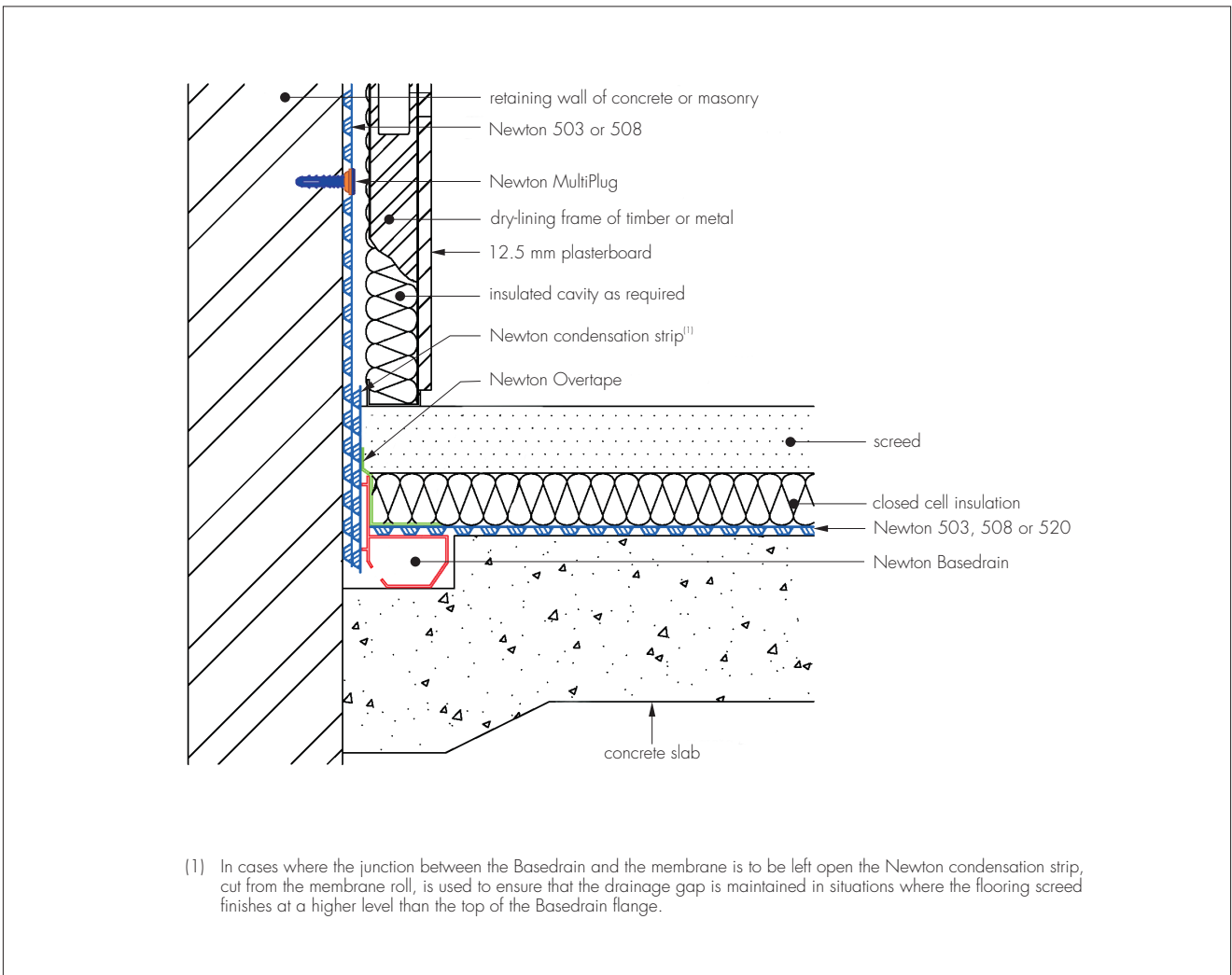
Figure 2 Installation detail
