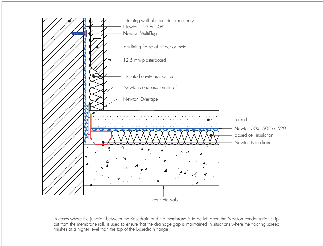
Figure 3 Installation detail
