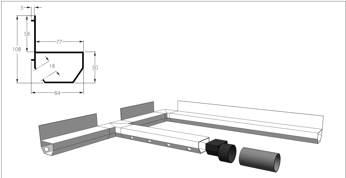
Figure 1 Newton Basedrain (all dimensions in mm)
