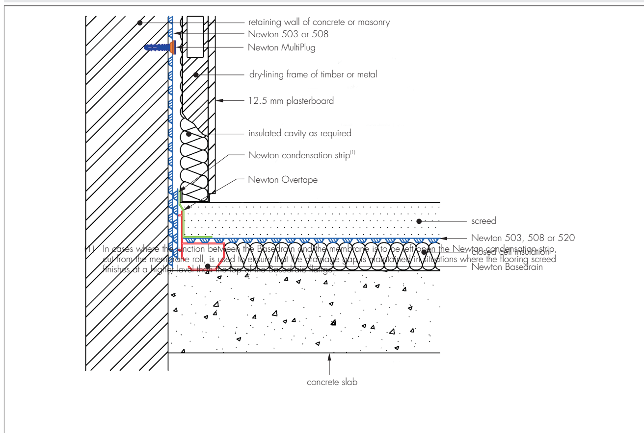
Figure 3 Installation detail
