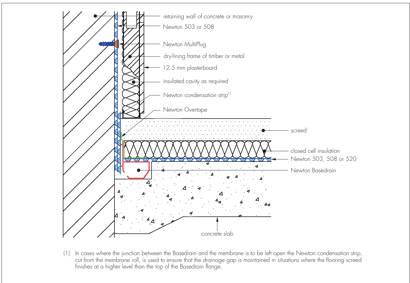
Figure 2 Installation detail — cut channel
